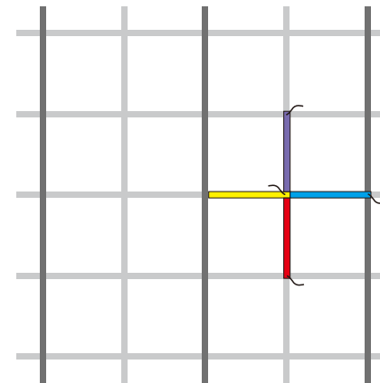
Main Tee Cross Tee Main Tee Cross Tee Main Tee
