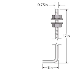
Anchor Bolt for 10ft,15ft,20ft,25ft
