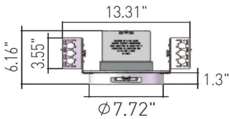
8" Housing
