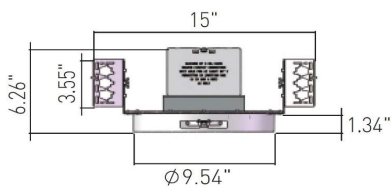
10" Housing
