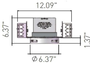
6" Housing
